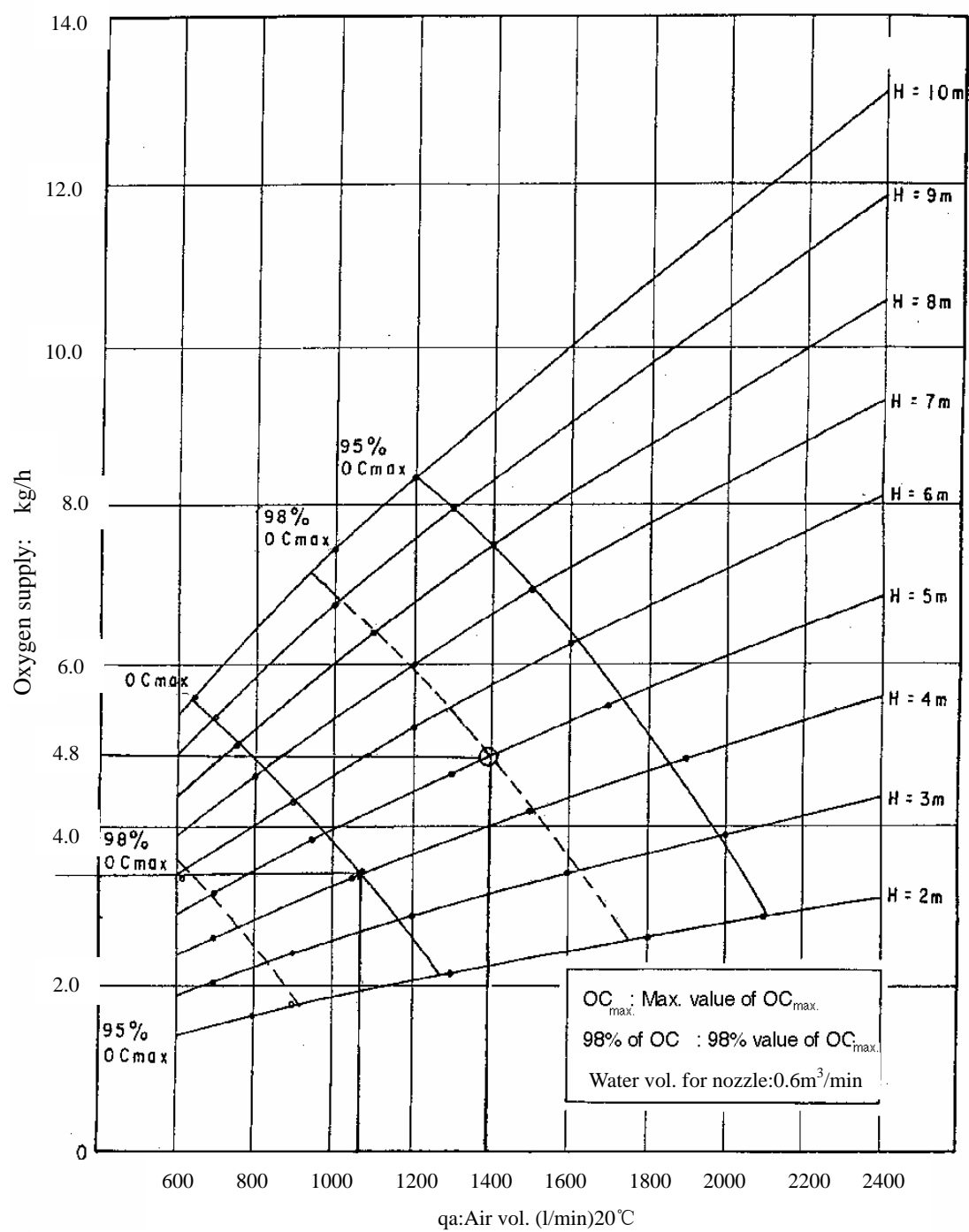
Figure: Oxygen supply vol. for nozzle applied to aeration tank
